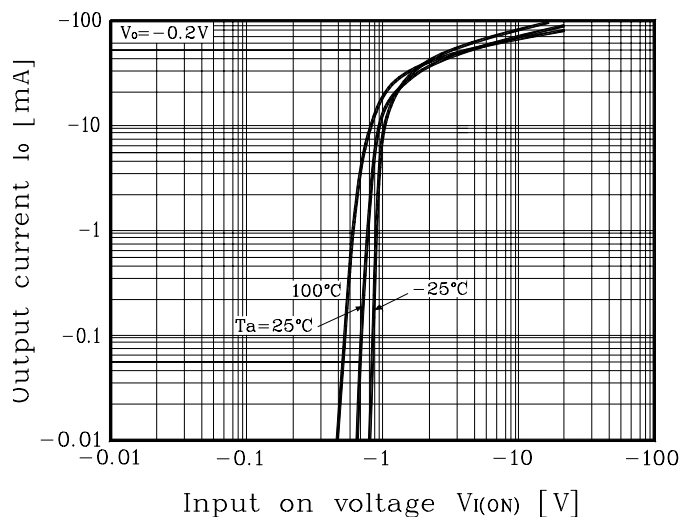
Fig. 2 I_O - V_{I(ON)}
