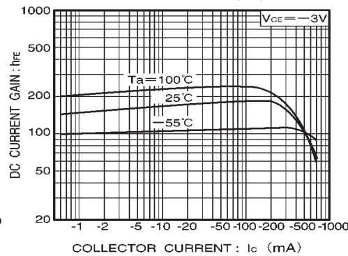
Fig.5 DC current gain vs. collector current ( II )
