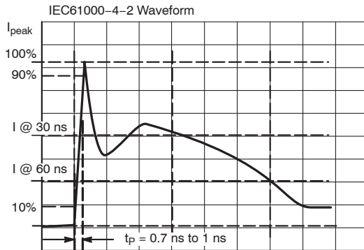
Figure 3. IEC61000-4-2 Spec
