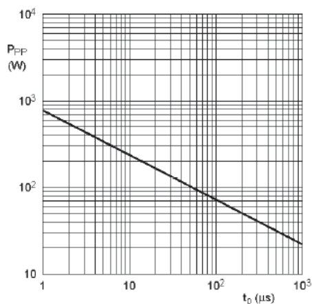
Peak pulse power as a function of exponential pulse duration; typical values
