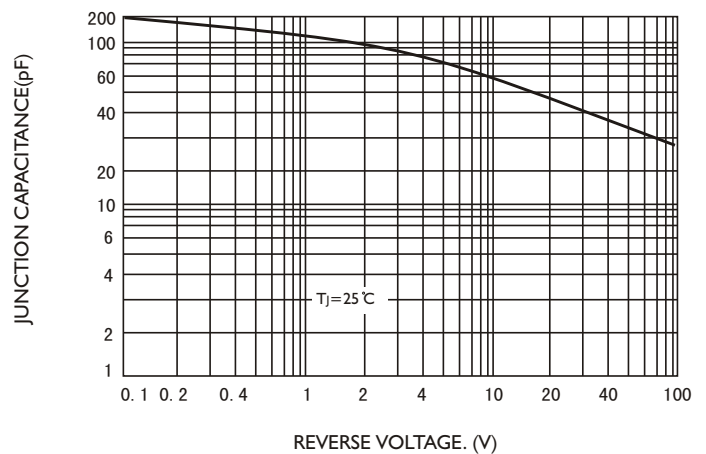
FIG.6-TYPICAL JUNCTION CAPACITANCE
