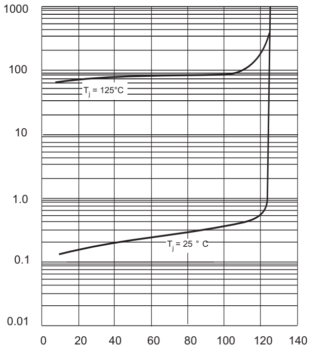
PERCENT OF RATED PEAK REVERSE VOLTAGE (%) Fig. 4 Typical Reverse Characteristics
