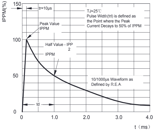
FIG3: PULSE WAVEFORM
