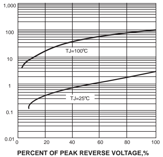
FIG. 4-TYPICAL REVERSE CHARACTERISTICS
